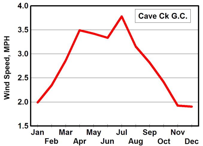
Figure 7. Annual trend of wind speed at Cave Creek Golf Course in Phoenix, AZ.
